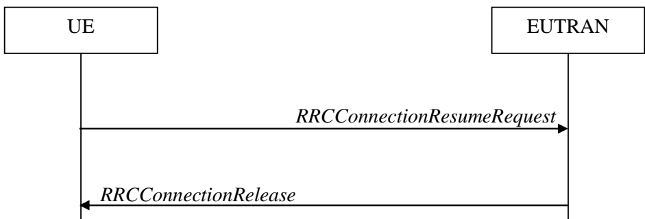
Figure 5.3.3.1-6: RRC connection resume (RRC_INACTIVE), network release or suspend or UP-EDT, successful
