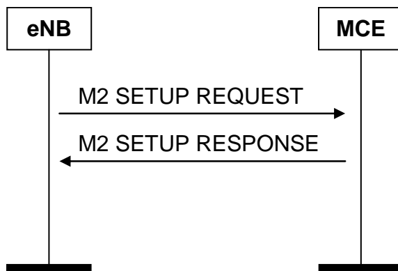
Figure 8.6.2-1. M2 Setup procedure. Successful operation.
