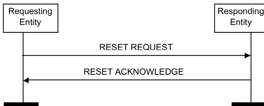
Figure 8.3.2.3.1.1: Crossing of Reset Messages.
