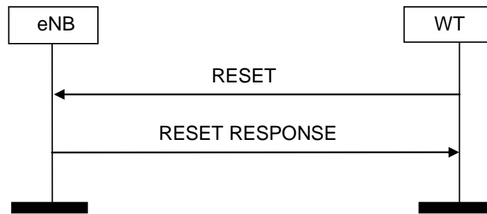
Figure 8.7.2-2: Reset, WT-initiated. Successful operation.
