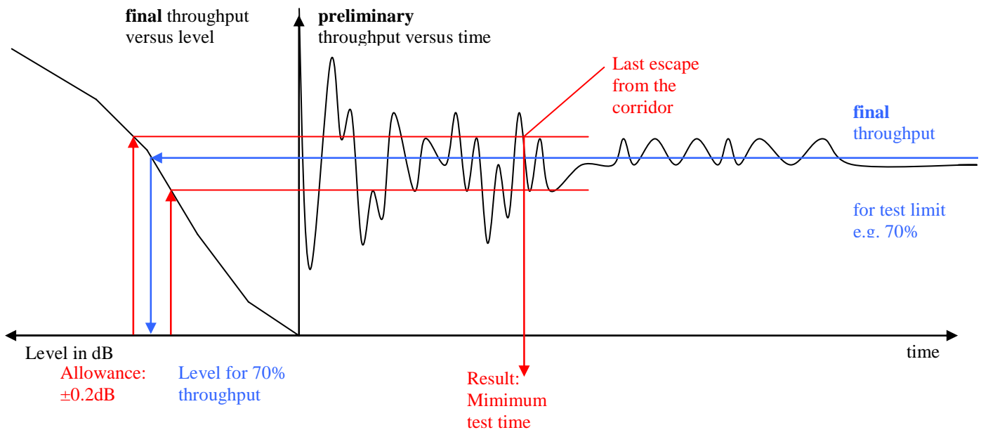
Fig. G.3.5-1: Simulation method to derive minimum test time
