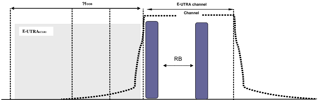
Figure 6.6.2.3_1.3-1: Adjacent Channel Leakage Power Ratio requirements
