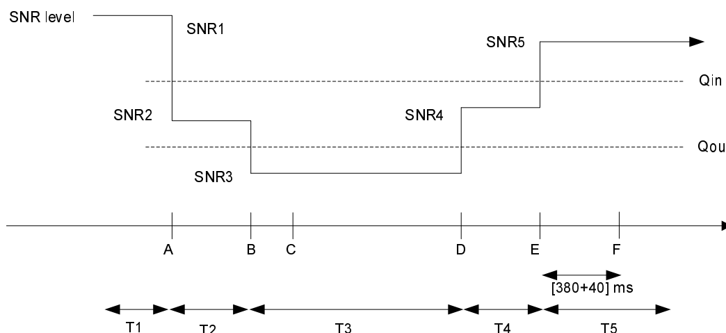
Figure 7.3.24.4-1: SNR variation for in-sync testing
