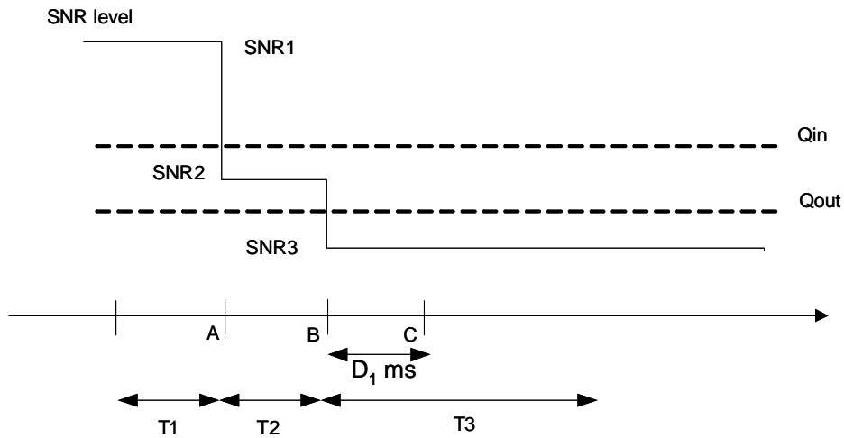
Figure 7.3.5.4-1: SNR variation for out-of-sync testing in DRX
