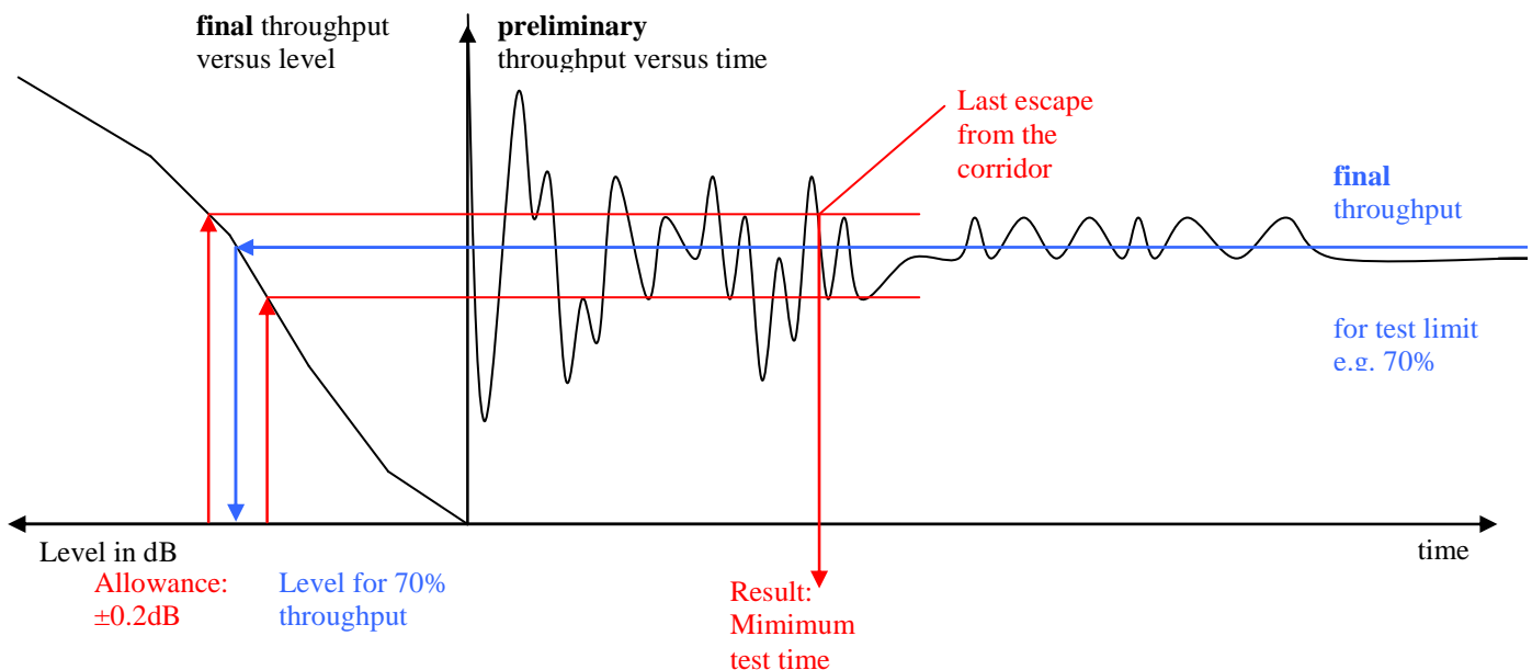
Figure G.3.5-1: Simulation method to derive minimum test time
