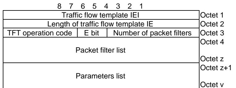
Figure 10.5.144/3GPP TS 24.008: Traffic flow template information element
