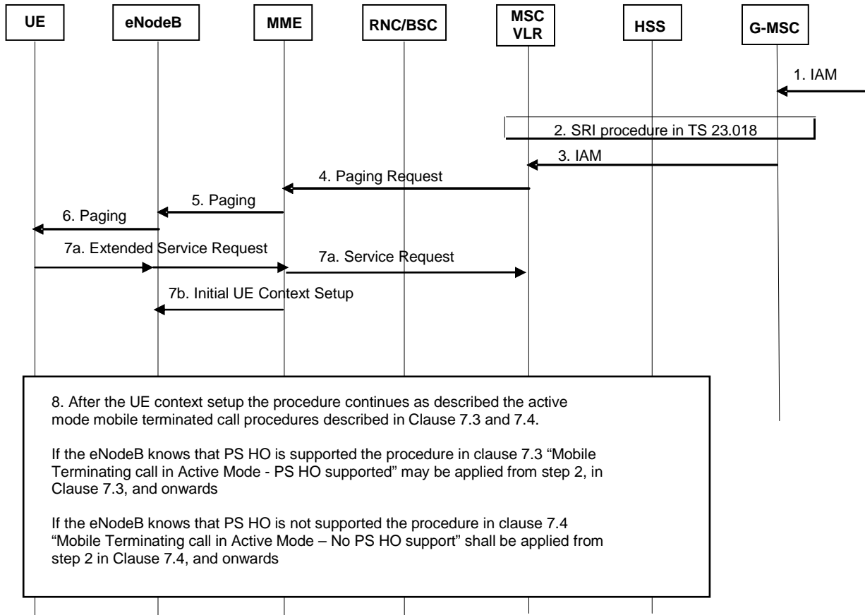
Figure 7.2-1: Mobile Terminating Call in idle mode
