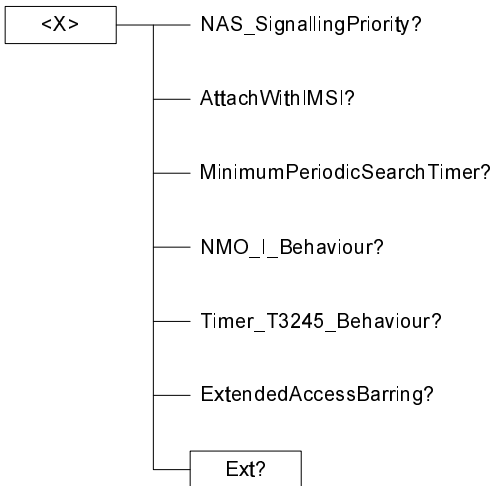
Figure 4-1: The NAS configuration Management Object
