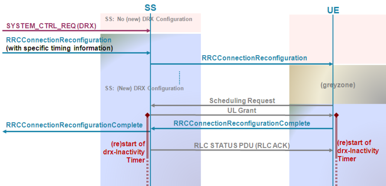
Figure 7.15-1: DRX (Re)configuration
