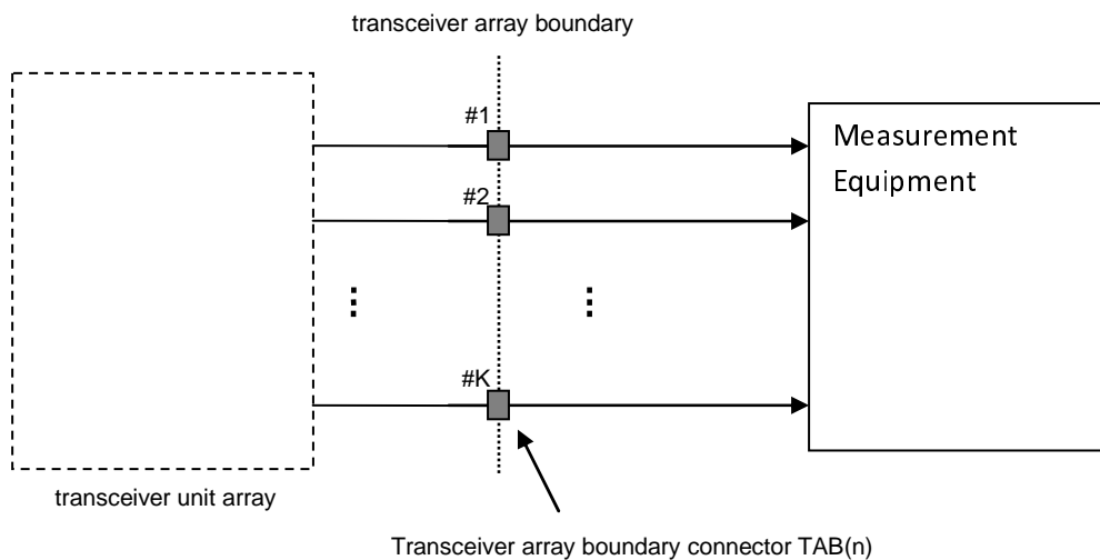
Figure D.1.1-2: Measuring system set-up for base station output power, transmitter ON/OFF power, modulation quality, transmitter spurious emissions and operating band unwanted emissions for multiple TAB connectors
