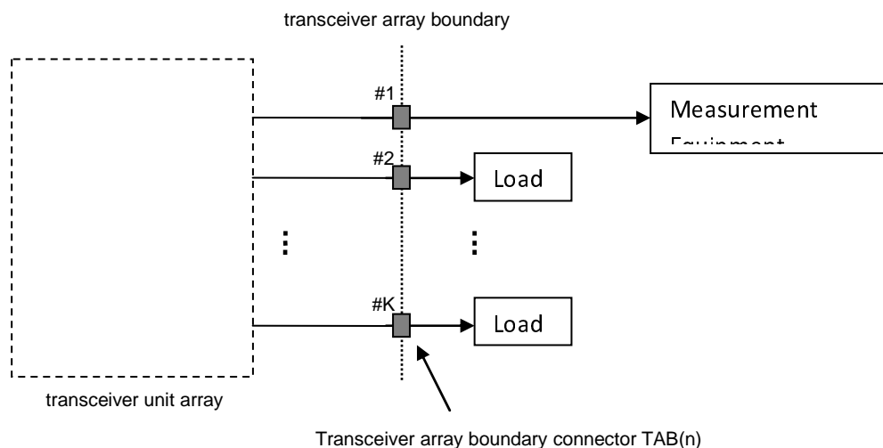
Figure D.1.1-1: Measuring system set-up for base station output power, transmitter ON/OFF power, modulation quality, transmitter spurious emissions and operating band unwanted emissions for a single TAB connector
