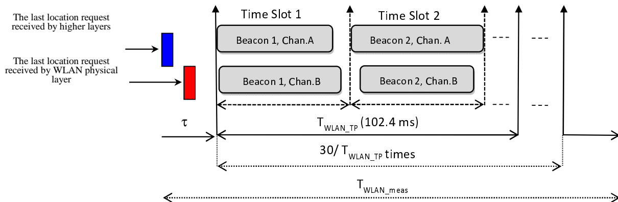
Figure 4.3.2.1.3-1: WLAN Measurement Time
