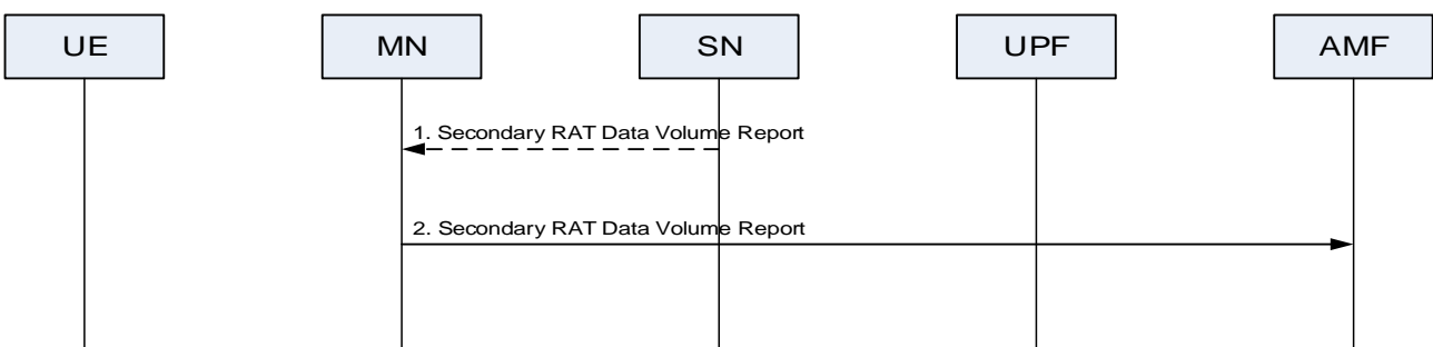
Figure 10.11.2-1: Secondary RAT data volume periodic reporting - MR-DC with 5GC
