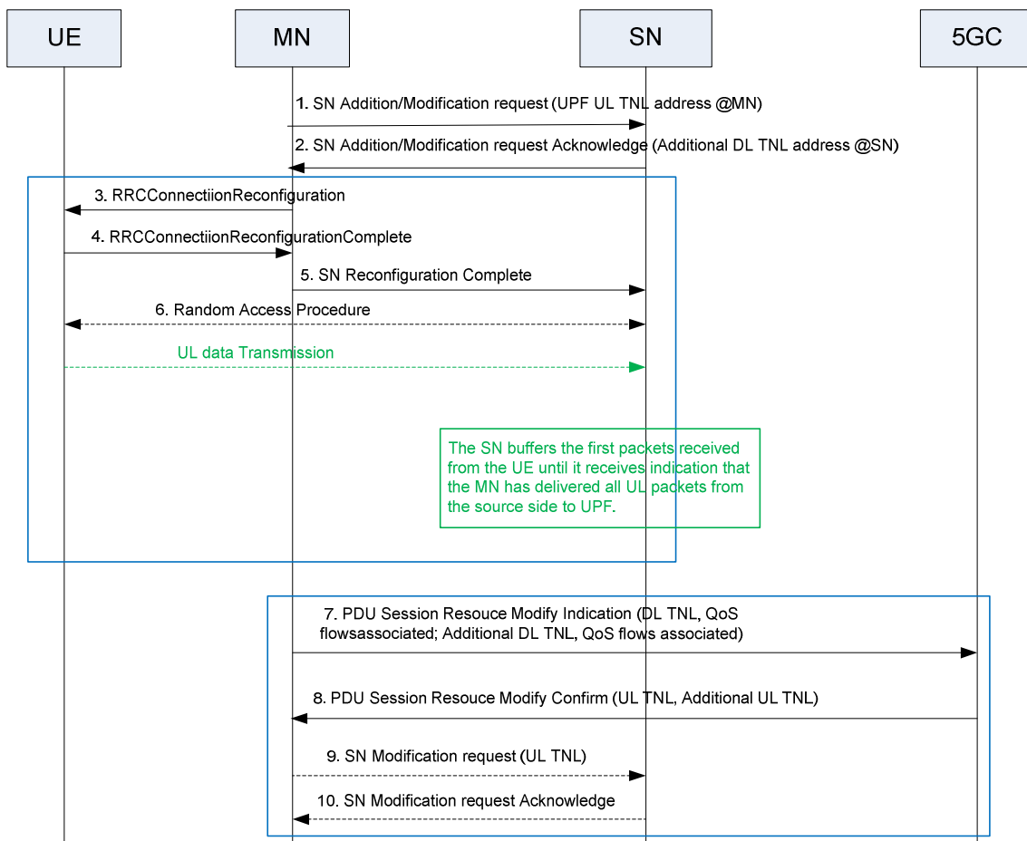
Figure 10.14.3-1: PDU Session Split at UPF during RAN initiated PDU session resource modify
