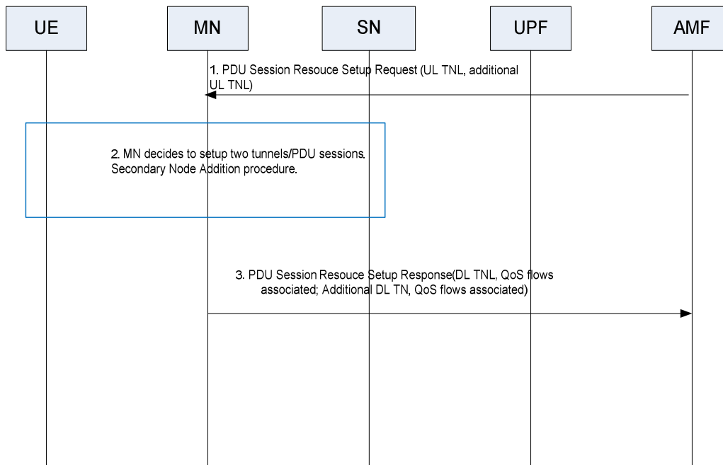
Figure 10.14.1-1: PDU Session Split at UPF during PDU session resource setup
