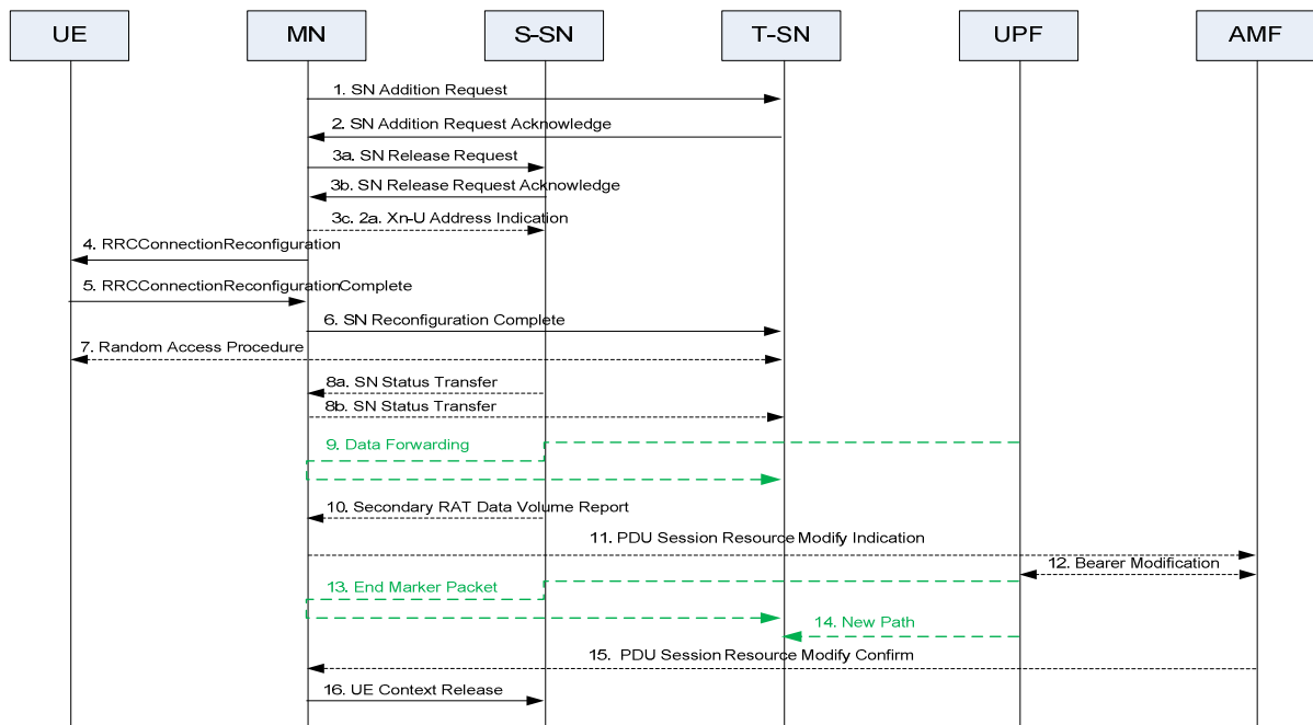
Figure 10.5.2-1: SN change procedure - MN initiated
