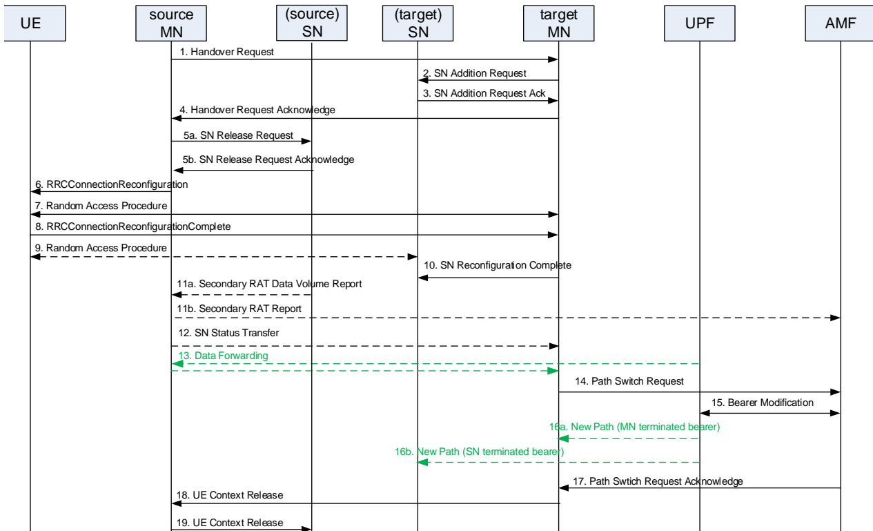
Figure 10.7.2-1: Inter-MN handover with/without MN initiated SN change procedure
