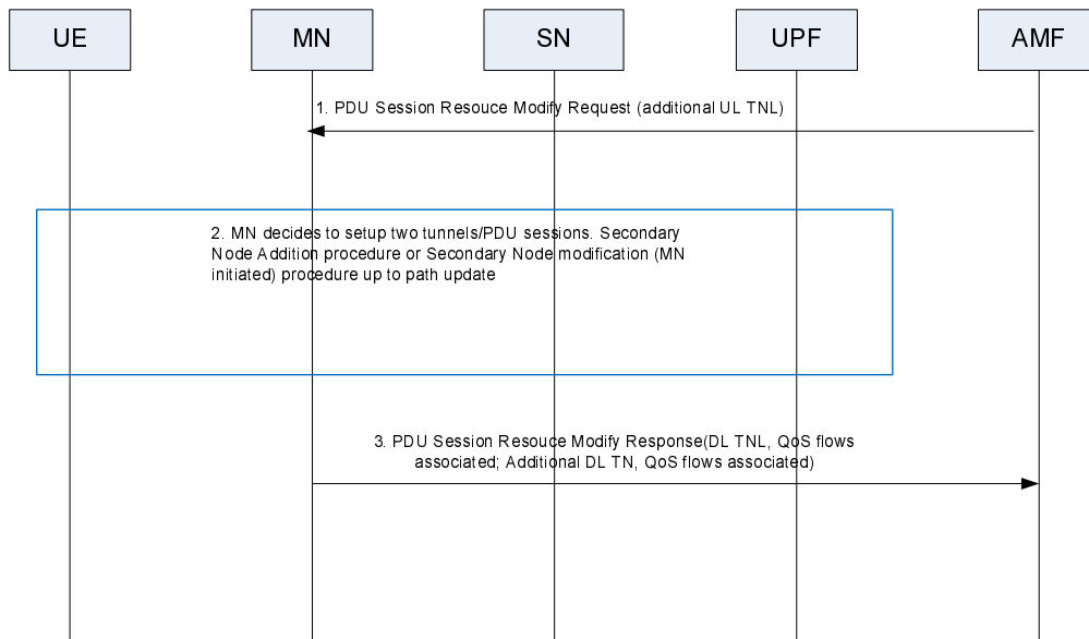
Figure 10.14.2-1: PDU Session Split at UPF during PDU session resource modify
