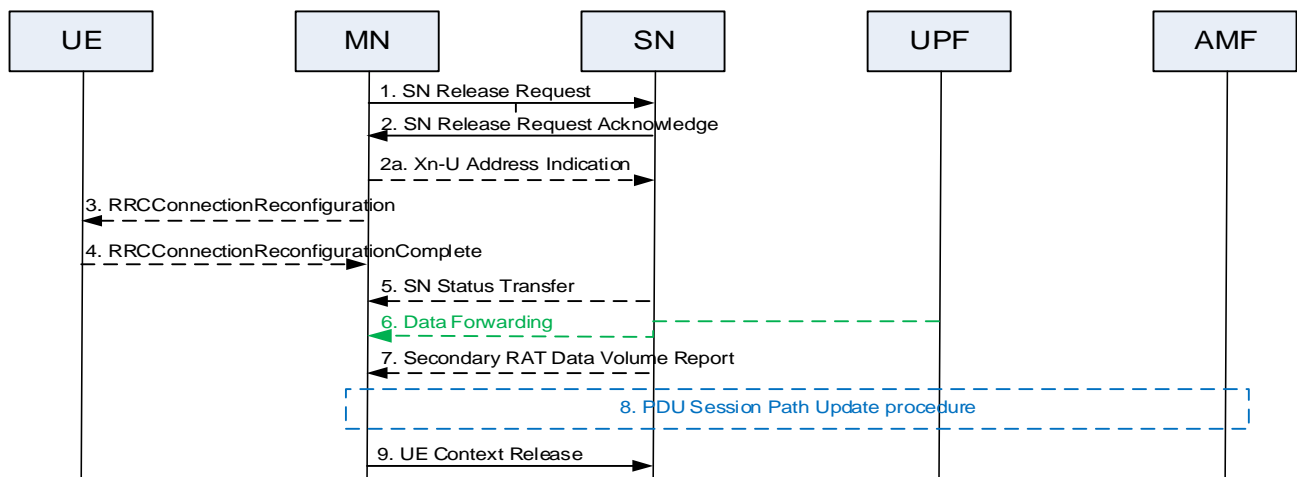
Figure 10.4.2-1: SN release procedure - MN initiated
