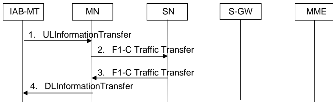
Figure 10.15-1: F1-C Traffic Transfer procedure in EN-DC
