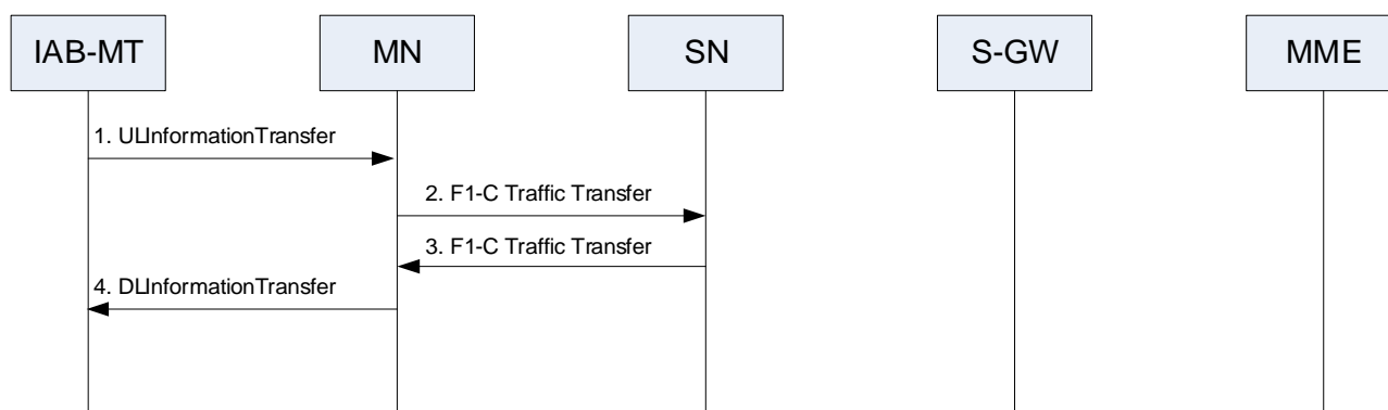
Figure 10.15-1: F1-C transfer procedure in EN-DC
