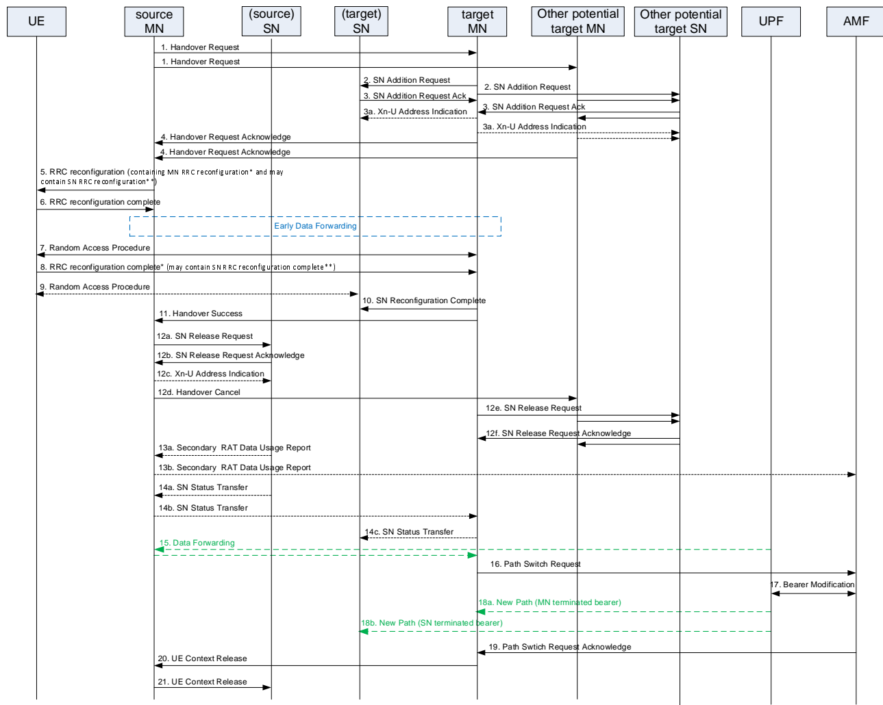
Figure 10.19.2-1: Conditional Handover with Secondary Node procedure
