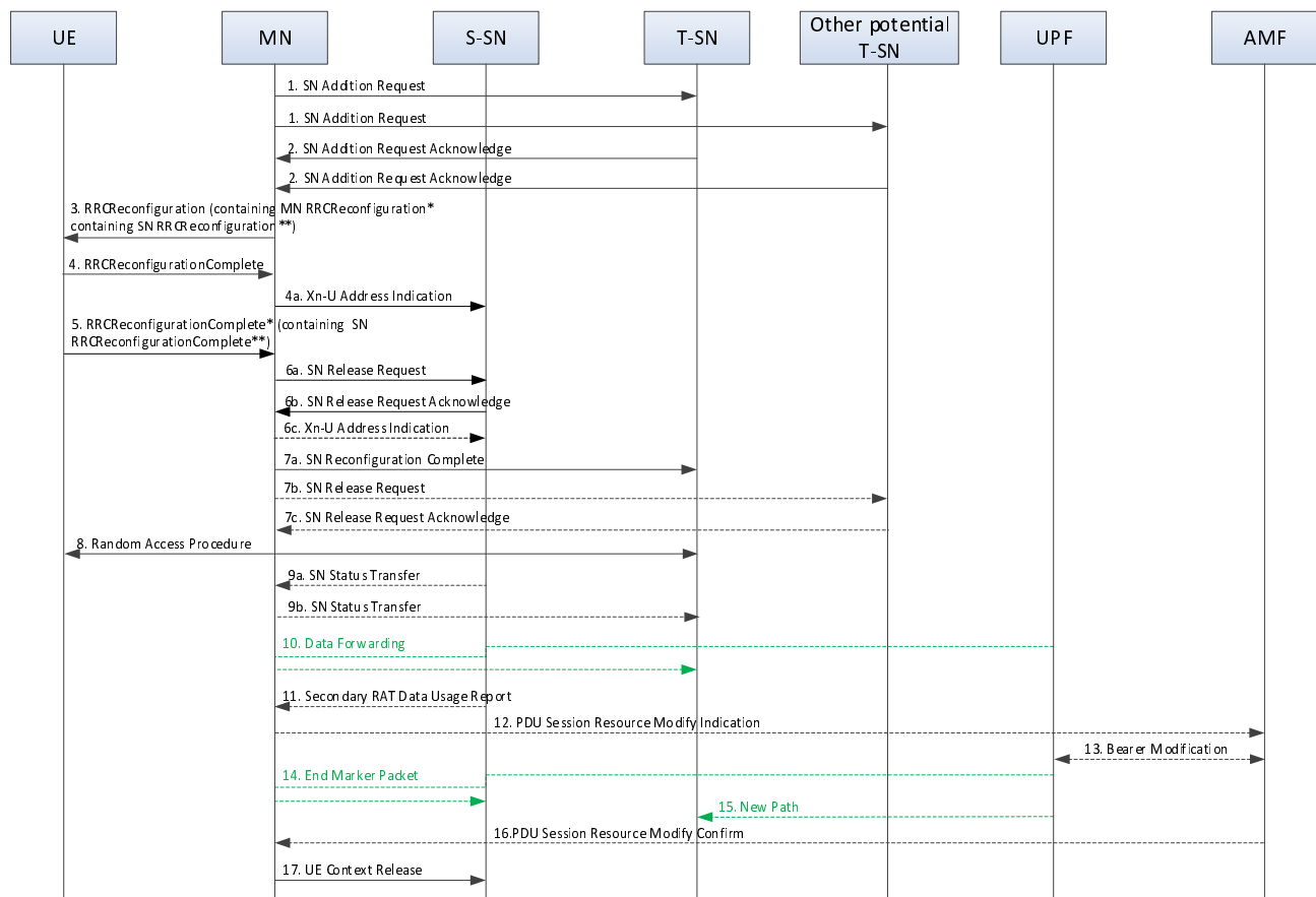
Figure 10.5.2-3: Conditional SN change procedure - MN initiated
