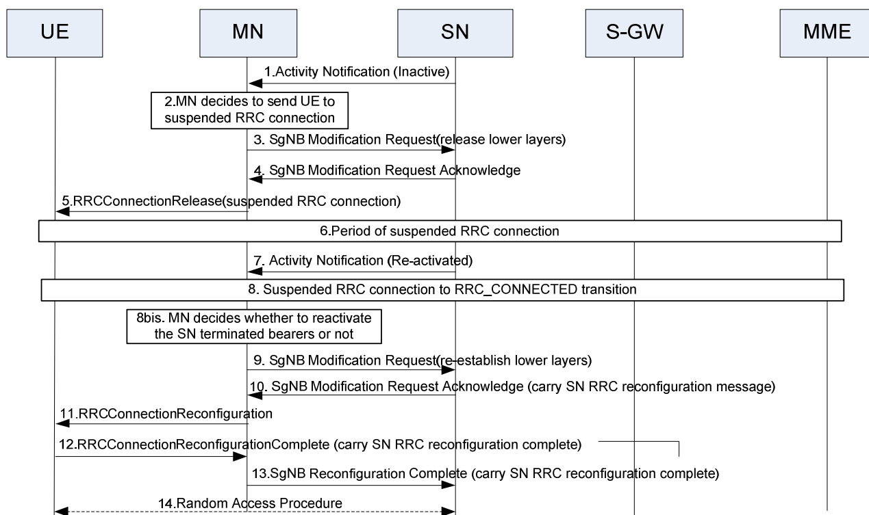
Figure 10.12.1-2: Support of Activity Notification in EN-DC with suspended RRC connection – SCG configuration released in SN
