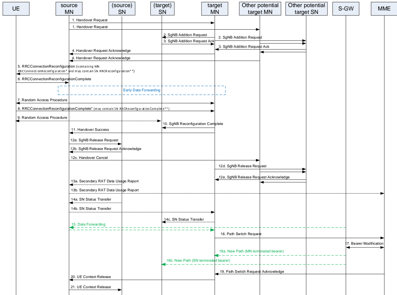
Figure 10.19.1-1: Conditional Handover with Secondary Node procedure
