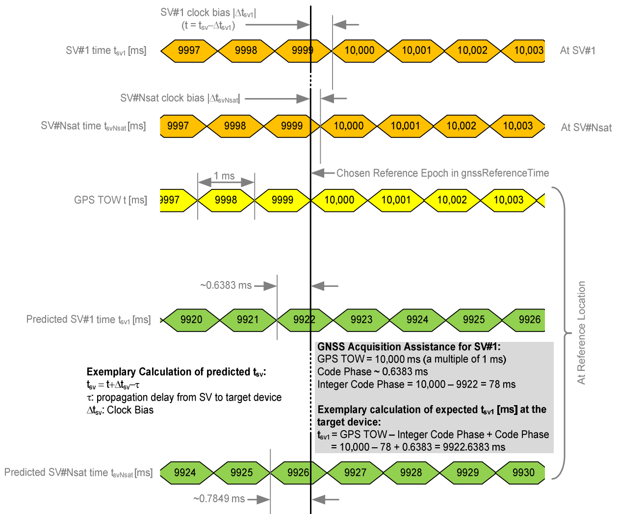
Figure 6.5.2.2-1: Exemplory calculation of some GNSS Acquisition Assistance fields.
