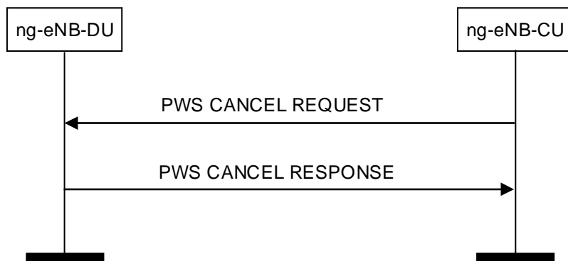
Figure 8.5.2.2-1: PWS Cancel procedure: successful operation
