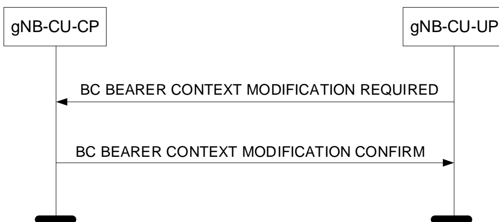
Figure 8.6.1.3.2-1: BC Bearer Context Modification procedure, gNB-CU-UP initiated: Successful Operation.
