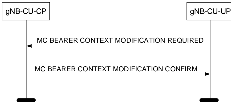
Figure 8.6.2.3.2-1: MC Bearer Context Modification procedure, gNB-CU-UP initiated: Successful Operation.
