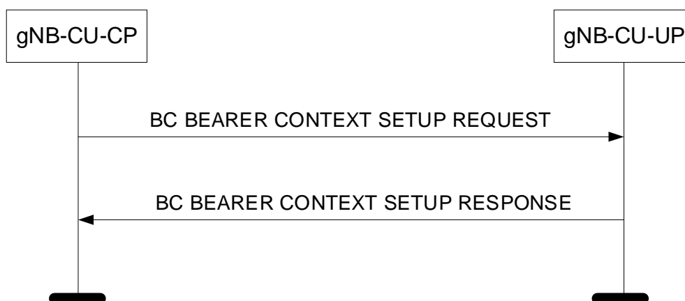
Figure 8.6.1.1.2-1: BC Bearer Context Setup procedure: Successful Operation.
