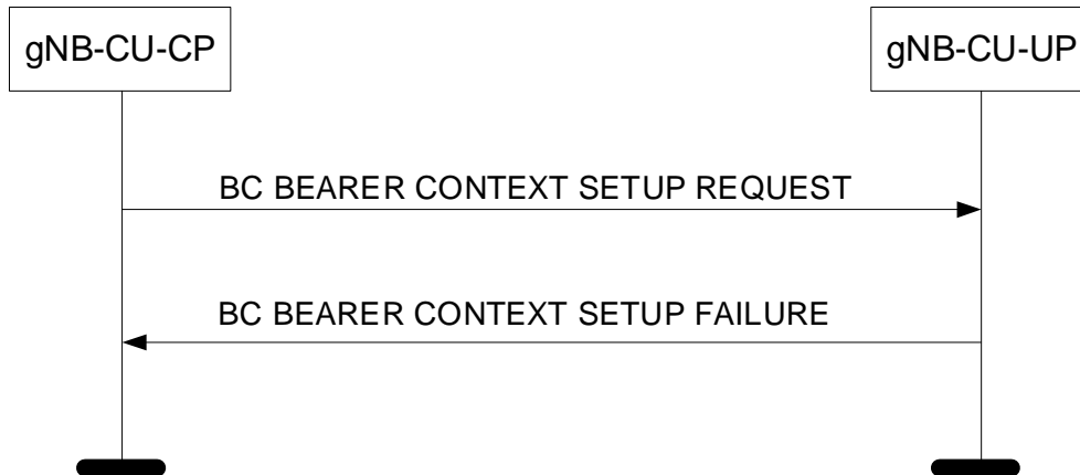
Figure 8.6.1.1.3-1: BC Bearer Context Setup procedure: Unsuccessful Operation.
