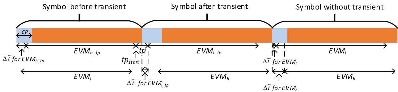
Figure F.4-1: EVM measurement window
