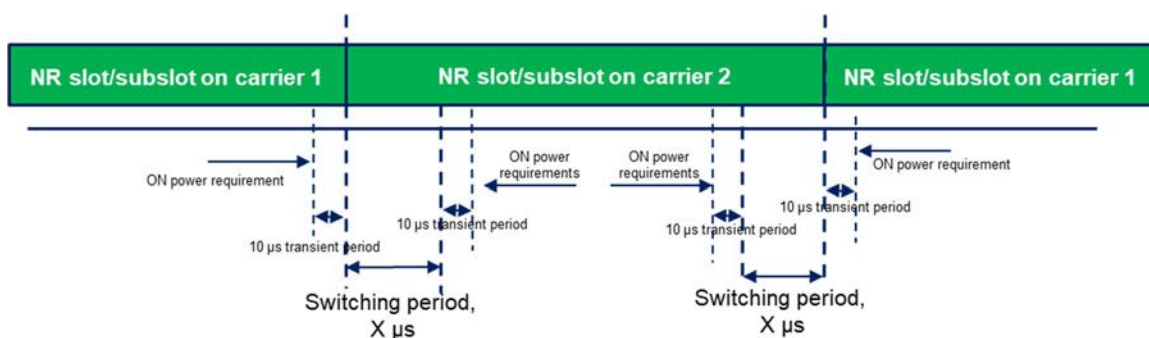
Figure 6.3C.3.2-1b: Time mask for switching between SUL carrier 1 and UL Carrier 2, where the switching period is located in carrier 2
