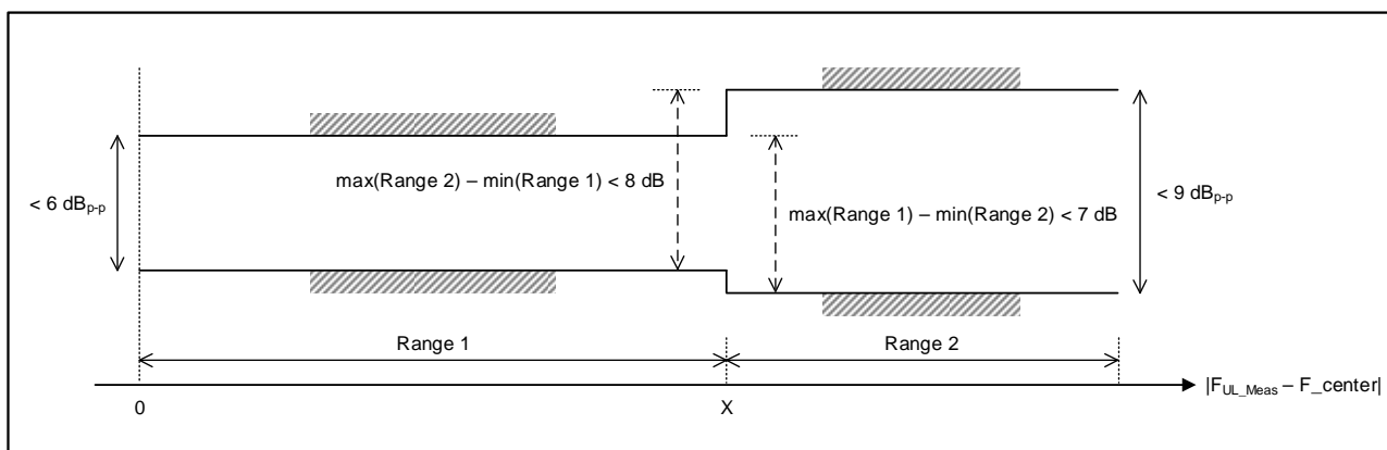
Figure 6.4.2.4-1: The limits for EVM equalizer spectral flatness with the maximum allowed variation of the coefficients indicated under normal conditions
