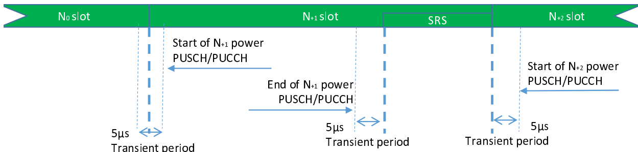
Figure 6.3.3.7-1: PUCCH/PUSCH/SRS time mask when there is a transmission before or after or both before and after SRS
