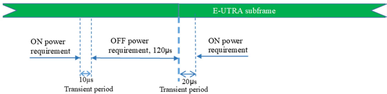
Figure 6.3B.2-2: NR to E-UTRA switching time mask for intra-band non-contiguous scenario
