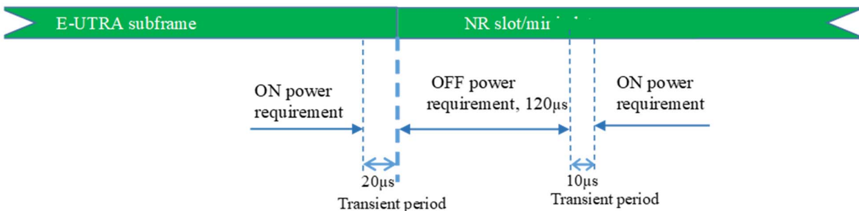
Figure 6.3B.2-1: E-UTRA to NR switching time mask for intra-band non-contiguous scenario
