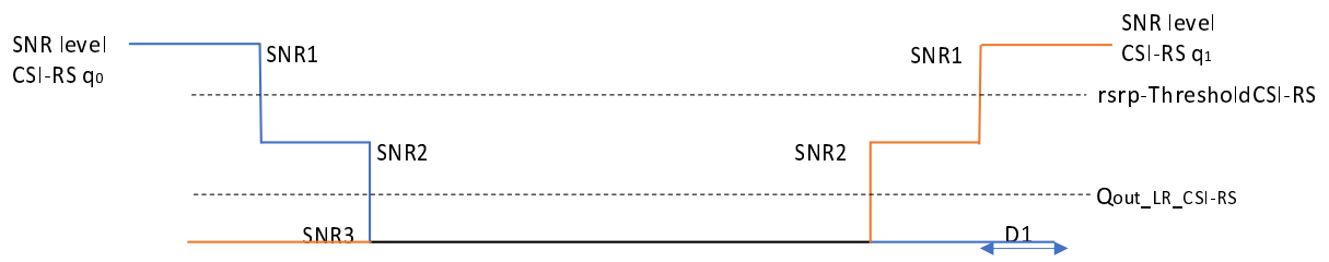
Figure A.6.5.5.3.1-1: SNR variation SSB for CSI-rs-based beam failure detection and link recovery testing in non-DRX mode
