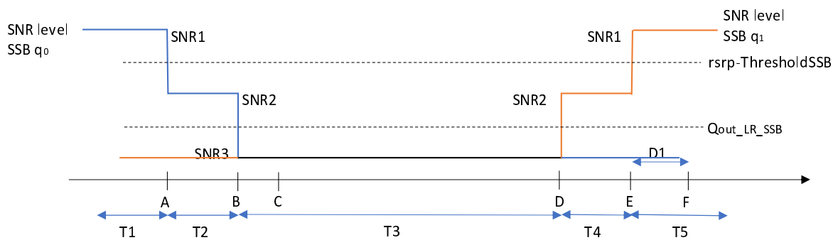
Figure A.5.5.2.1-1: SNR variation for SSB-based beam failure detection and link recovery testing in non-DRX mode
