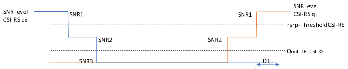
Figure A.6.5.5.4.1-1: SNR variation SSB for CSI-rs-based beam failure detection and link recovery testing in DRX mode
