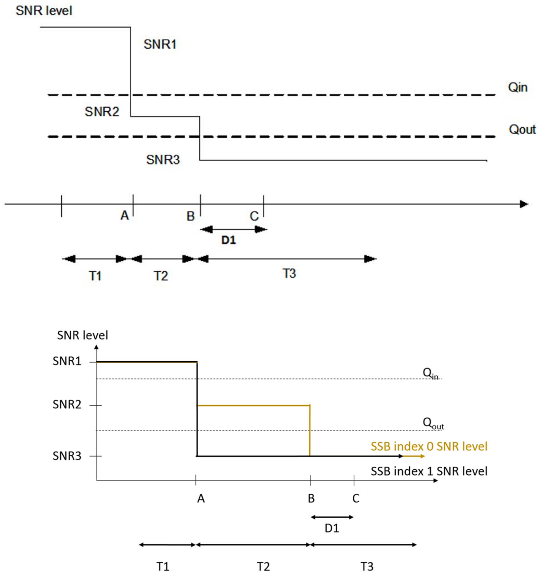
Figure A.7.5.1.1.1-1: SNR variation for out-of-sync testing
