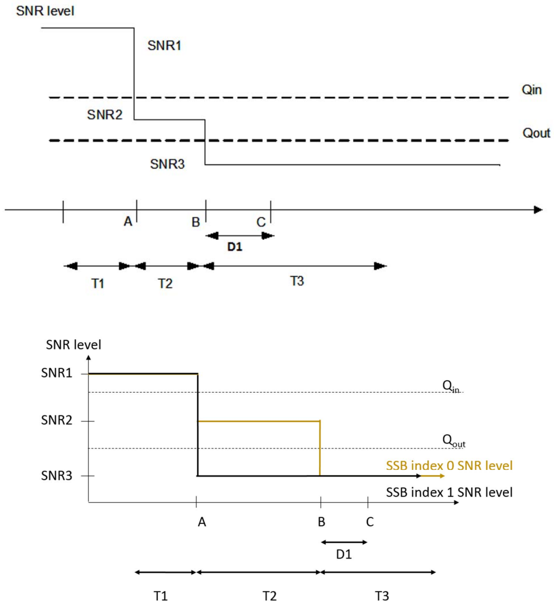
Figure A.7.5.1.3.1-1: SNR variation for out-of-sync testing
