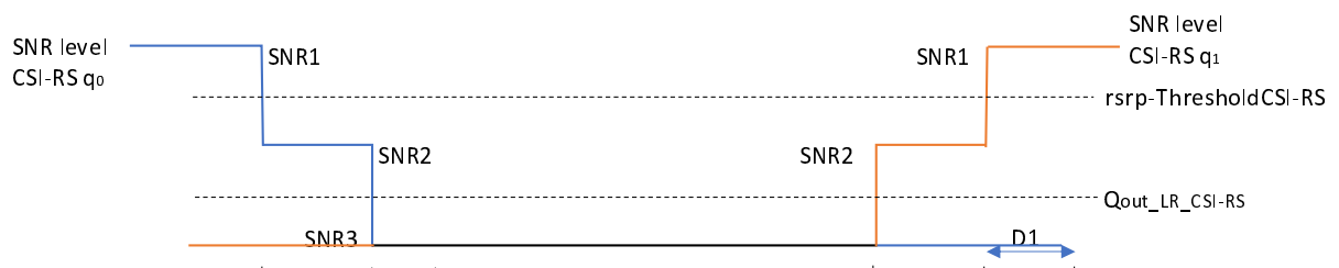
Figure A.7.5.5.3.1-1: SNR variation SSB for CSI-RS based beam failure detection and link recovery testing in non-DRX mode
