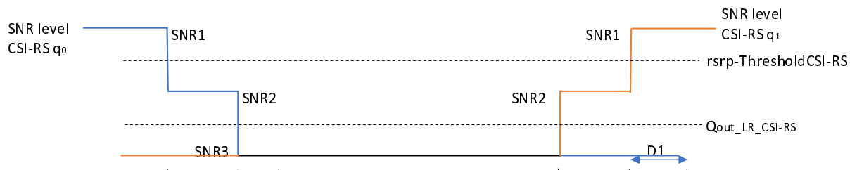
Figure A.4.5.5.3.1-1: SNR variation SSB for CSI-RS-based beam failure detection and link recovery testing in non-DRX mode
