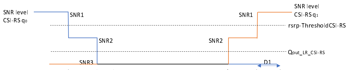
Figure A.5.5.3.1-1: SNR variation SSB for CSI-RS based beam failure detection and link recovery testing in non-DRX mode
