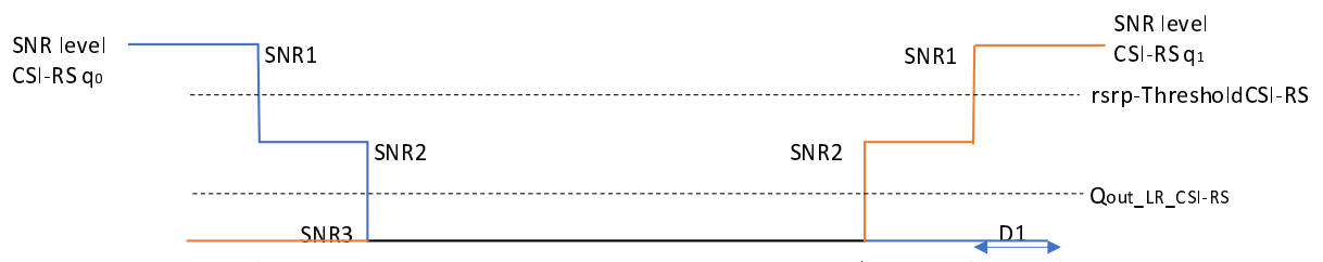
Figure A.4.5.1.4.1-1: SNR variation SSB for CSI-RS-based beam failure detection and link recovery testing in DRX mode
