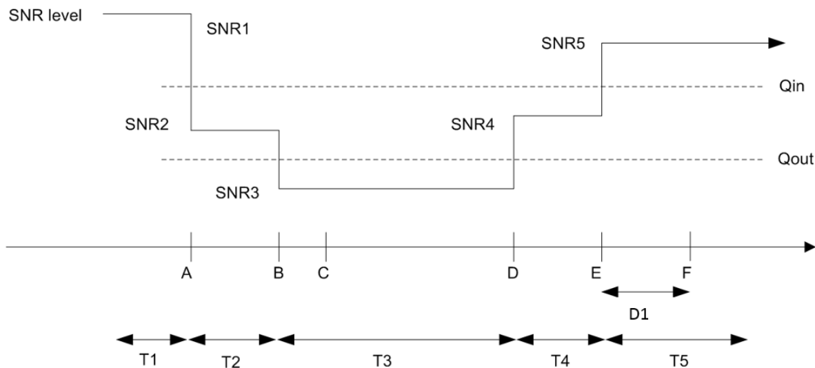
Figure A.6.5.1.2.1-1: SNR variation for in-sync testing
