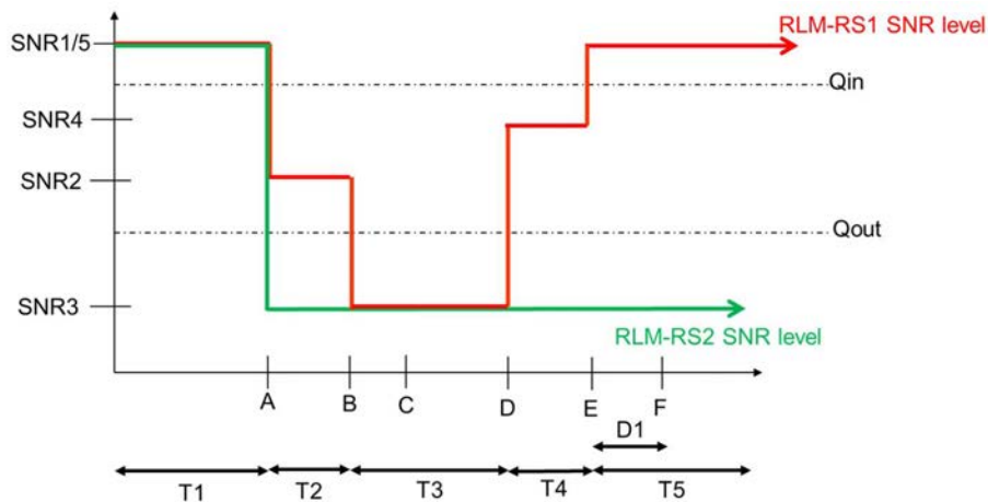
Figure A.7.5.1.6.1-1: SNR variation for CSI-RS in-synch testing
