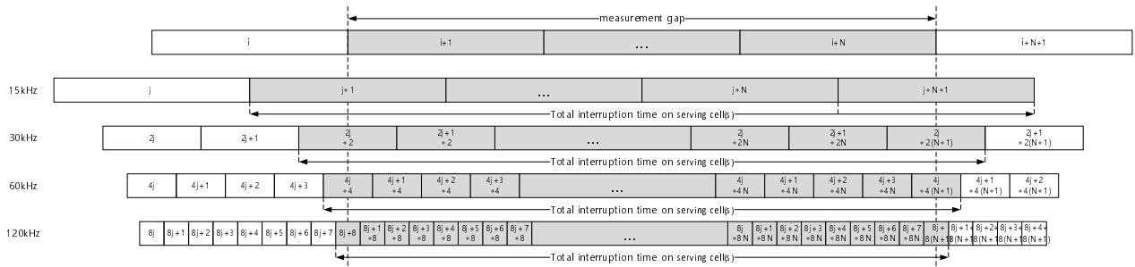
(c) Measurement gap with MGL = N(\text{ms}) with MG timing advance of 0ms for all serving cells in asynchronous EN-DC and asynchronous NE-DC, and for serving cells in SCG in NR standalone operation (with asynchronous NR-DC configuration)
