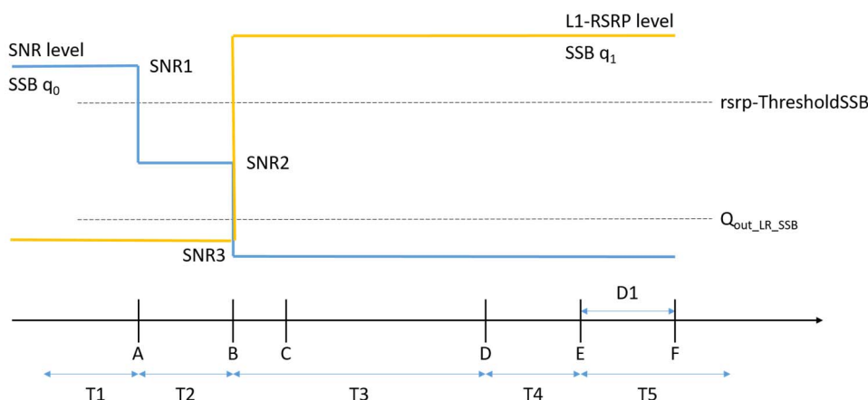
Figure A.4.5.5.2.1-1: SNR and L1-RSRP variation for SSB-based beam failure detection and link recovery testing in non-DRX mode
