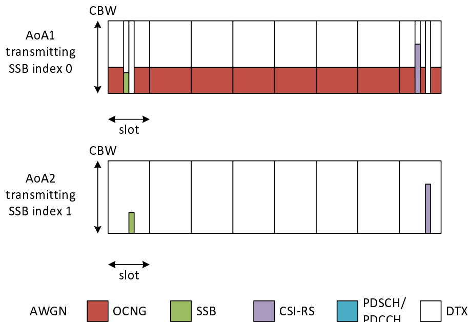
Figure A.7.6.1.1-1: Time multiplexed downlink transmissions (Config 1 example)
