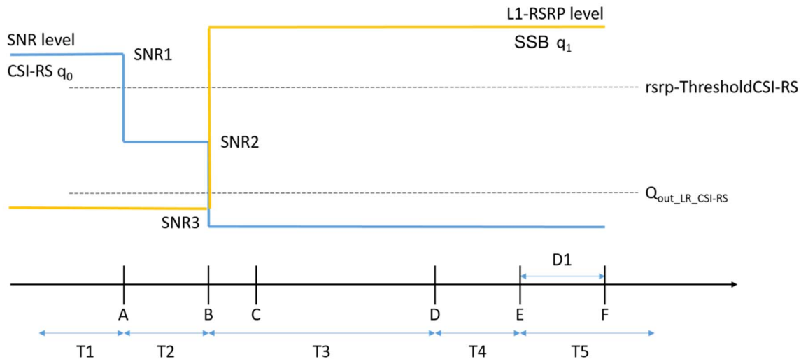
Figure A.6.5.5.5.1-1: SNR and L1-RSRP variation for beam failure detection and link recovery testing in for SCell non-DRX mode
