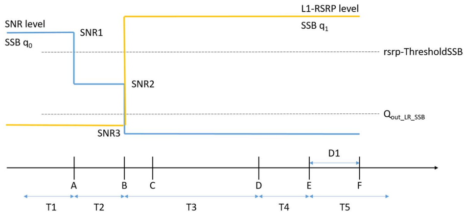
Figure A.11.4.4.1-1: SNR and L1-RSRP variation SSB for SSB-based beam failure detection and link recovery testing in non-DRX mode
