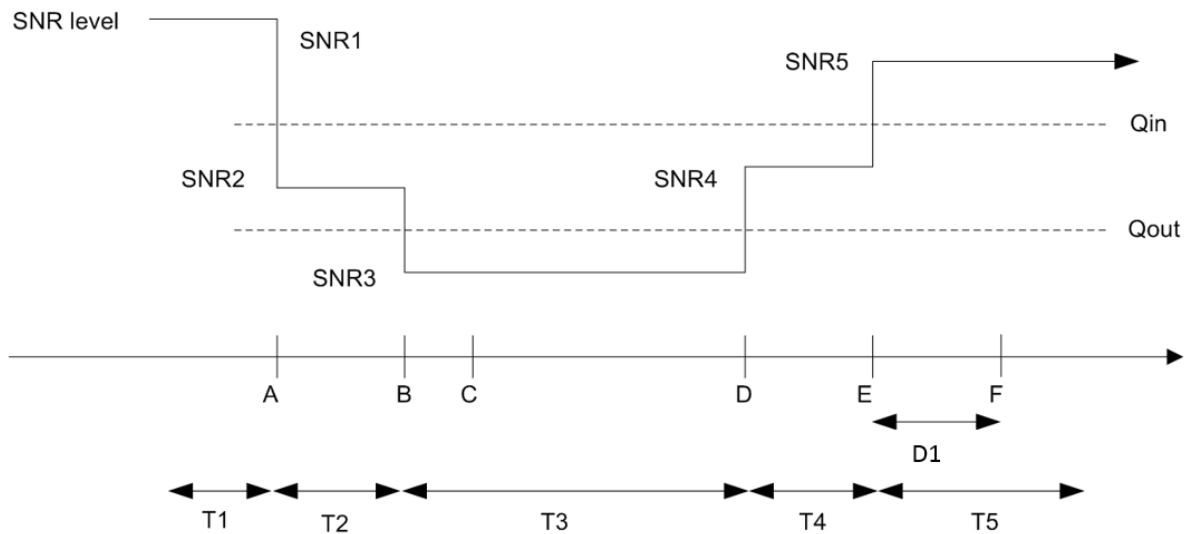
Figure A.6.5.1.2.1-1: SNR variation for in-sync testing
