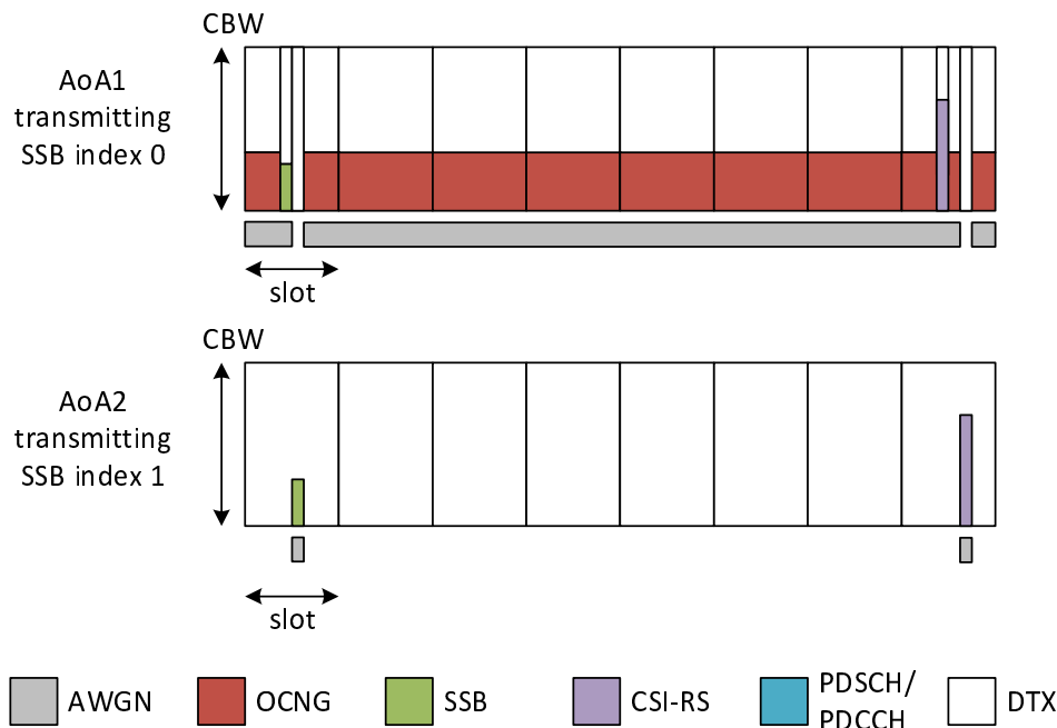
Figure A.7.5.1.1.1-2: Time multiplexed downlink transmissions
