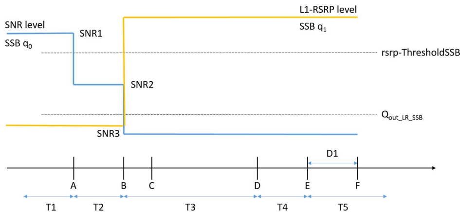
Figure A.6.5.5.1.1-1: SNR and L1-RSRP variation SSB for SSB-based beam failure detection and link recovery testing in non-DRX mode
