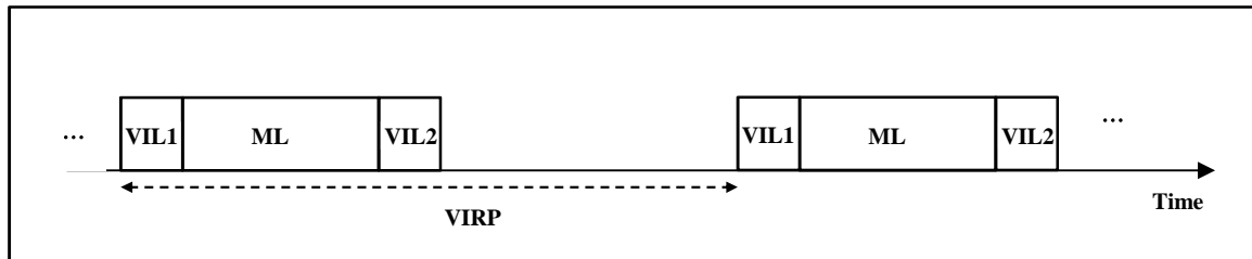
Figure 9.1.9-1: Illustration of NCSG configuration parameters: VIL1, ML, VIL2 and VIRP
