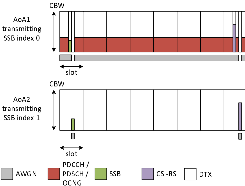
Figure G.2.3B.3.1.1-1: Time multiplexed downlink transmissions during T1
