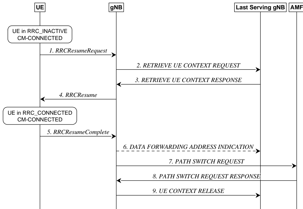
Figure 9.2.2.4.1-1: UE triggered transition from RRC_INACTIVE to RRC_CONNECTED (UE context retrieval success)
