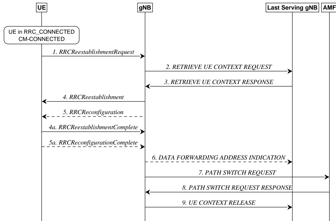
Figure 9.2.3.3-1: Re-establishment procedure
