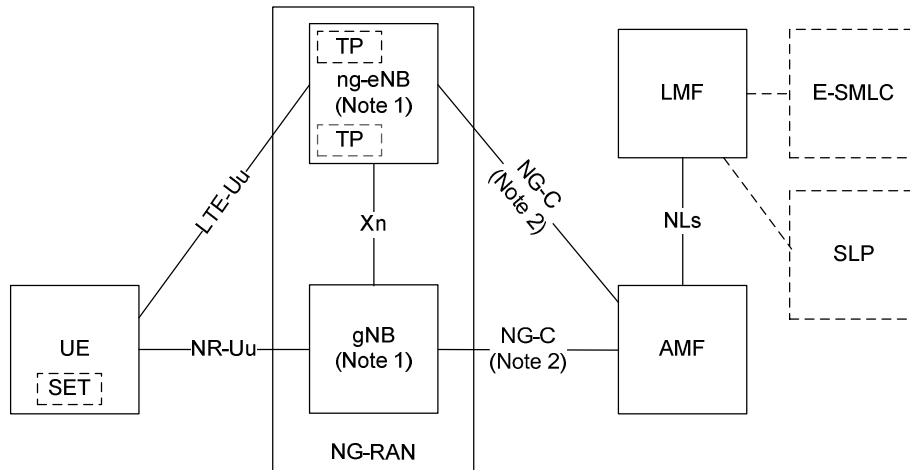
Figure 5.1-1: UE Positioning Architecture applicable to NG-RAN
