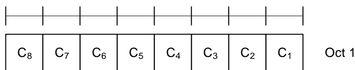
Figure 6.1.3.34-1: Sidelink Configured Grant Confirmation MAC CE
