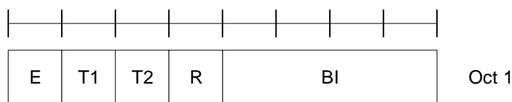
Figure 6.1.5a-1: BI MAC subheader
