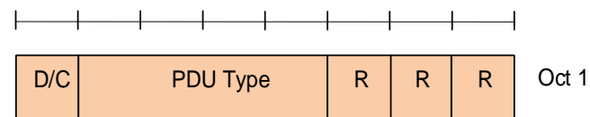
Figure 6.2.3.4-1: BAP Control PDU format for BH RLF detection indication
