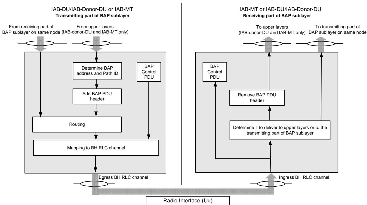
Figure 4.2.2-1. Example of functional view of BAP sublayer
