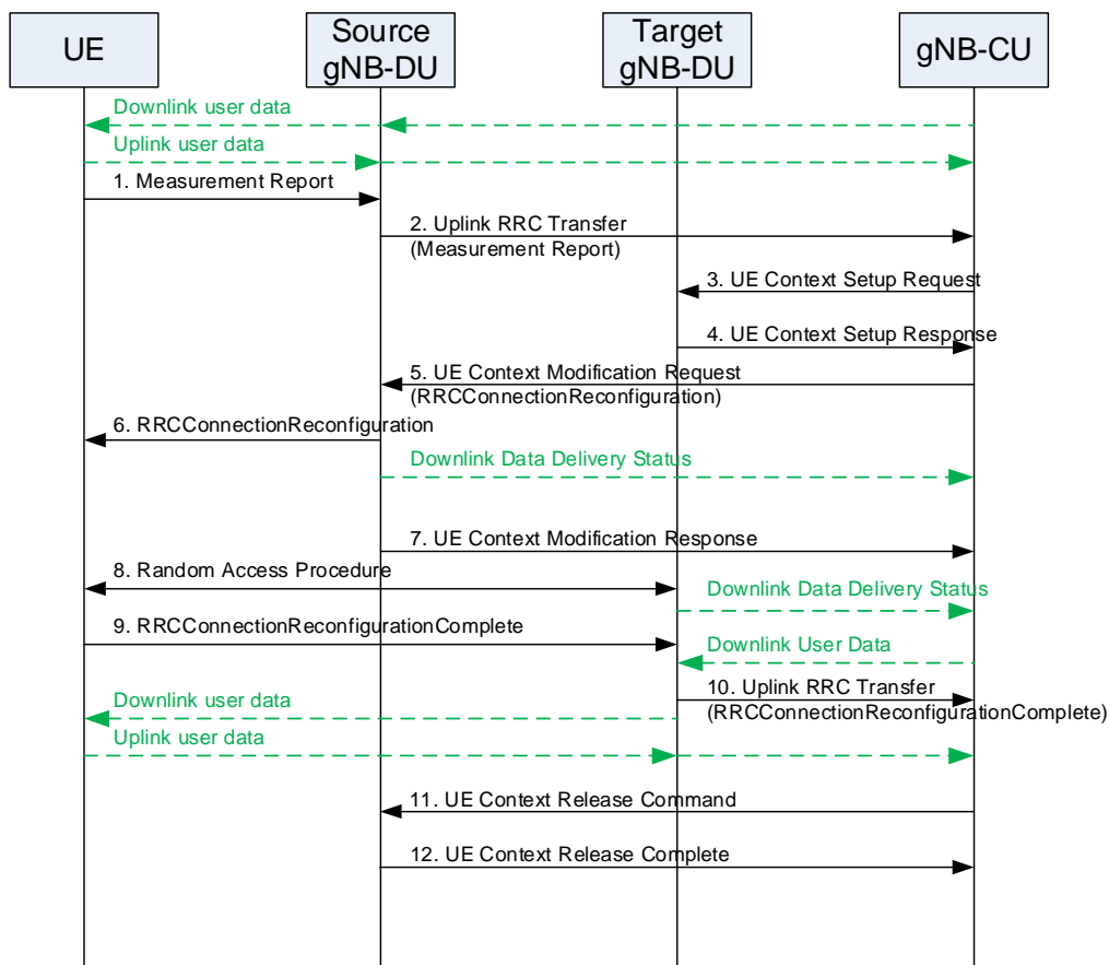
Figure 8.2.1.1-1: Inter-gNB-DU Mobility for intra-NR
