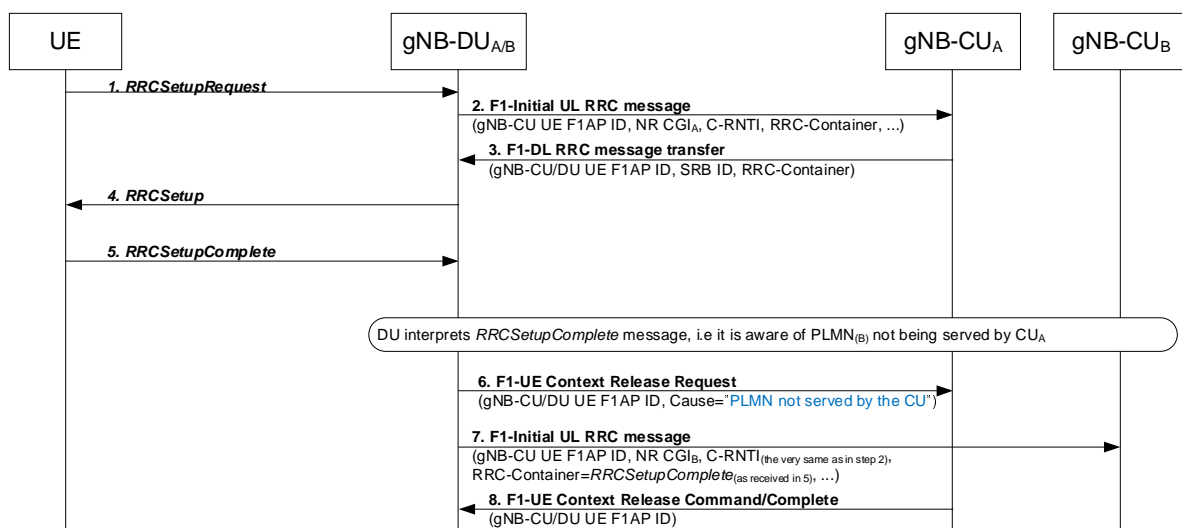
Figure 8.11.2-1: UE Initial Access procedure and network sharing with multiple cell-ID broadcast
