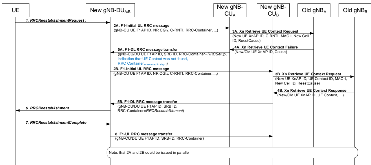
Figure 8.11.3-1: RRC Connection Reestablishment and network sharing with multiple cell-ID broadcast
