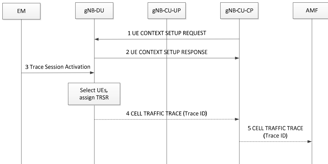
Figure 8.13.2-2 Management based MDT Activation in gNB-DU
