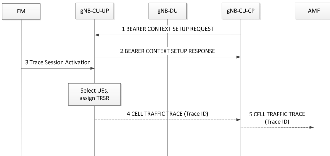
Figure 8.13.2-3 Management based MDT Activation in gNB-CU-UP
