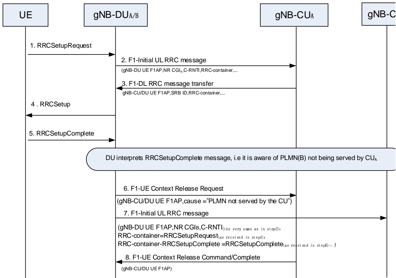
Figure 8.11.2-1: UE Initial Access procedure and network sharing with multiple cell-ID broadcast
