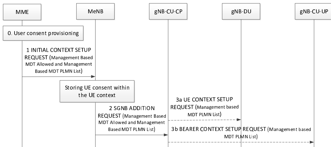
Figure 8.13.2-4 User consent propagation in EN-DC
