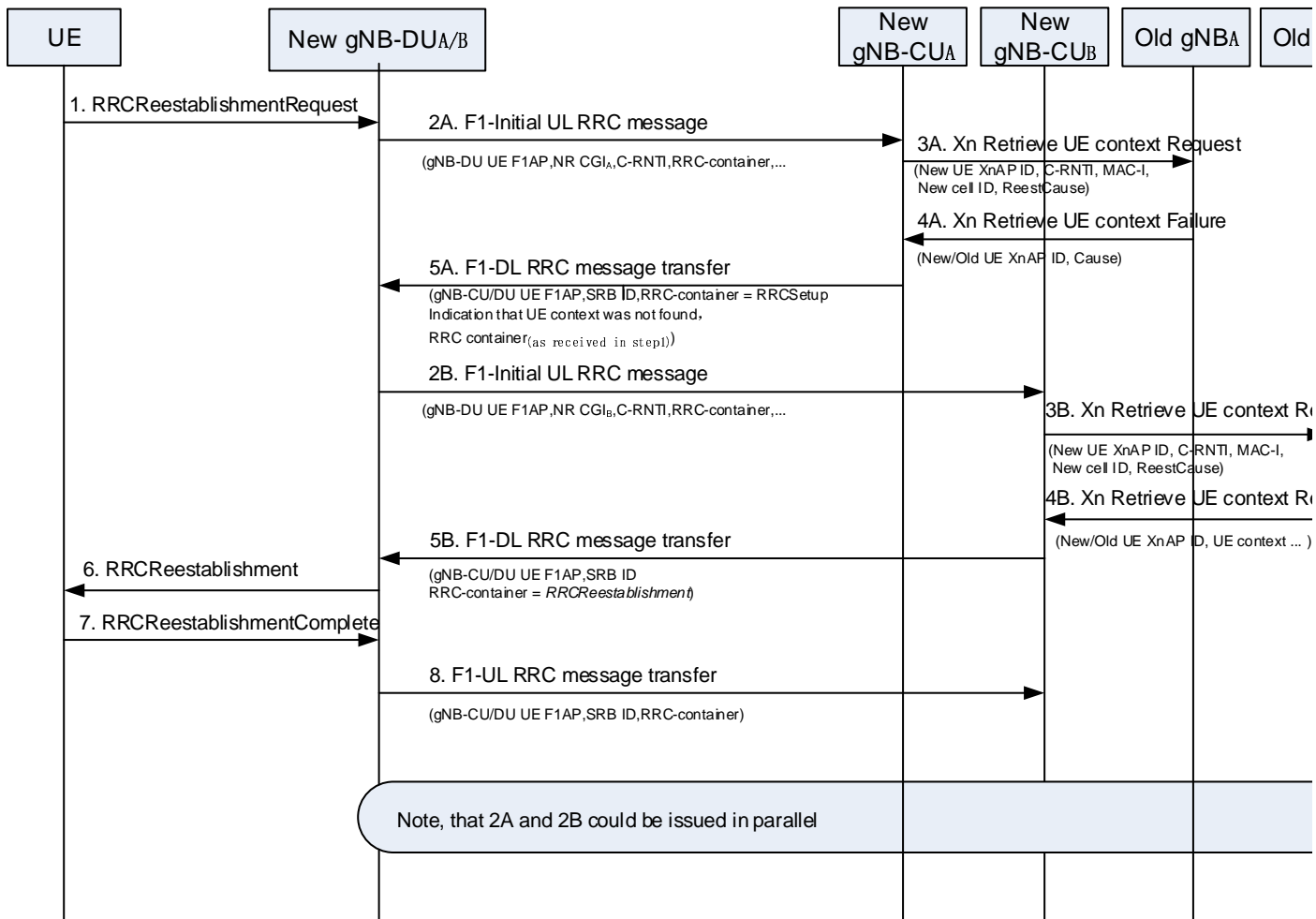
Figure 8.11.3-1: RRC Connection Reestablishment and network sharing with multiple cell-ID broadcast
