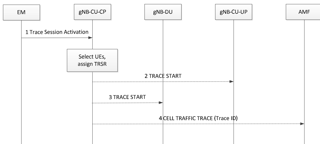
Figure 8.13.2-1 Management based MDT Activation in gNB-CU-CP
