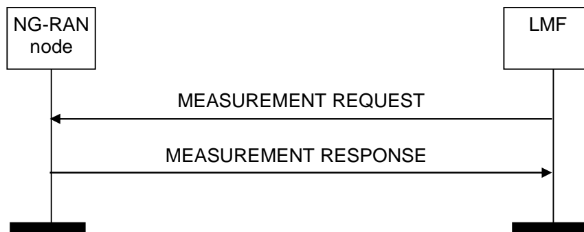
Figure 8.z.1.2.1: Measurement procedure. Successful operation.
