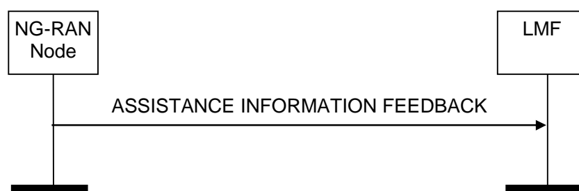
Figure 8.4.2.2-1: Assistance Information Feedback procedure
