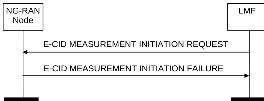
Figure 8.2.1.3-1: E-CID Measurement Initiation procedure, unsuccessful operation
