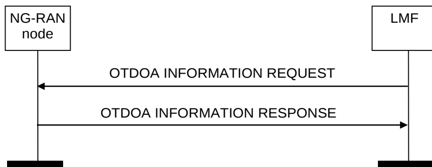
Figure 8.2.5.2-1: OTDOA Information Exchange procedure, successful operation
