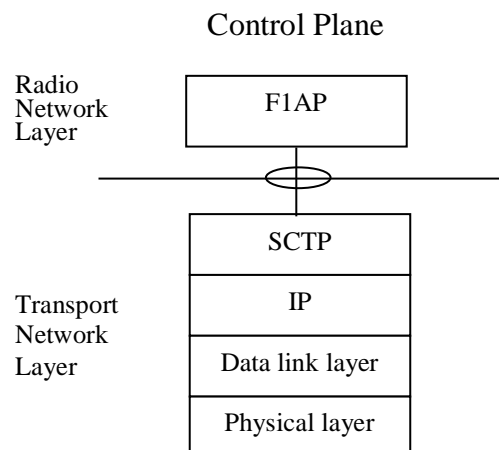
Figure 7.1-1: Interface protocol structure for F1-C
