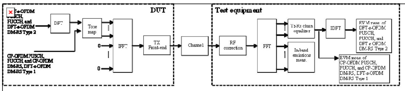
Figure E.2.5-1: EVM measurement points
