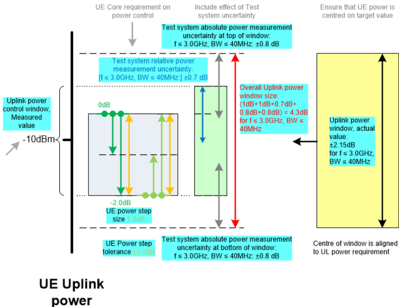
Figure F.4.4.3-1: Example E-UTRA uplink power setting centred on a target value
