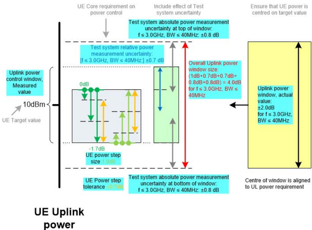
Figure F.4.4.1-1: Example NR FR1 uplink power setting centred on a target value
