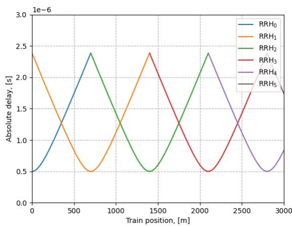
Figure B.3.6-5: Absolute delay trajectories
