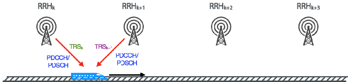
Figure B.3.5-1: Deployment of HST-SFN Scheme A
